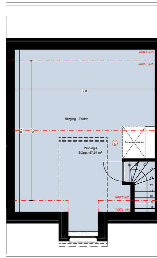
Zolder:
